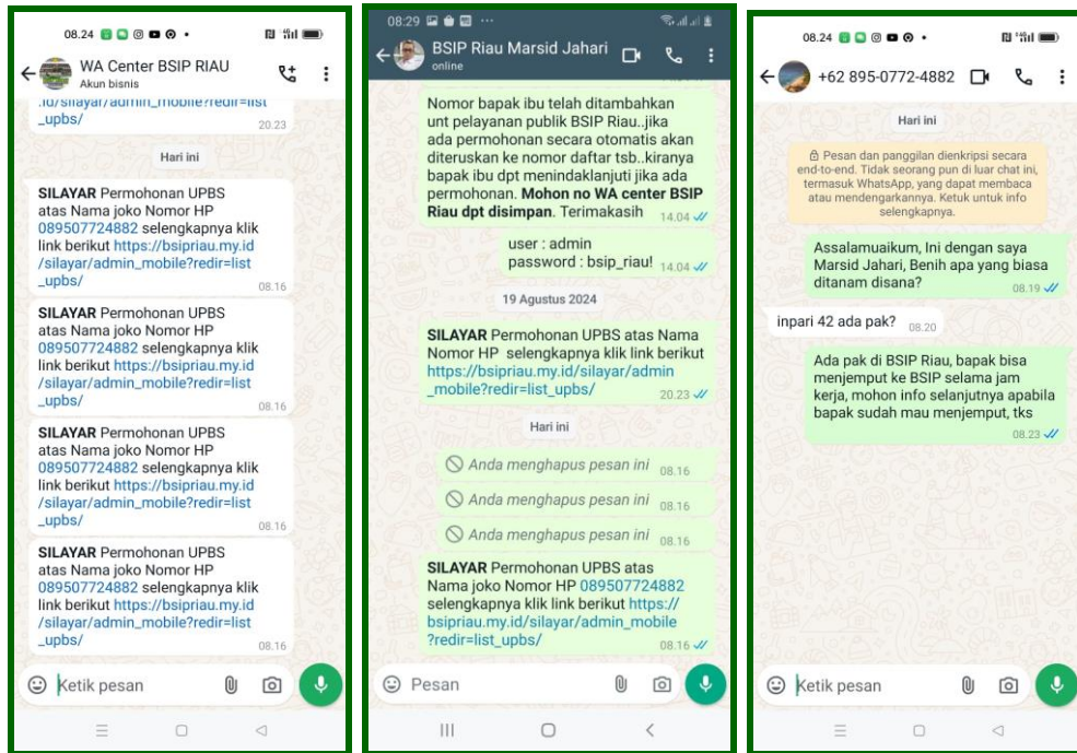
Gambar 32. Whatsapp Gateway
