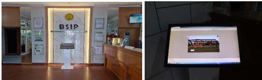
Gambar 11. Counter Layanan
